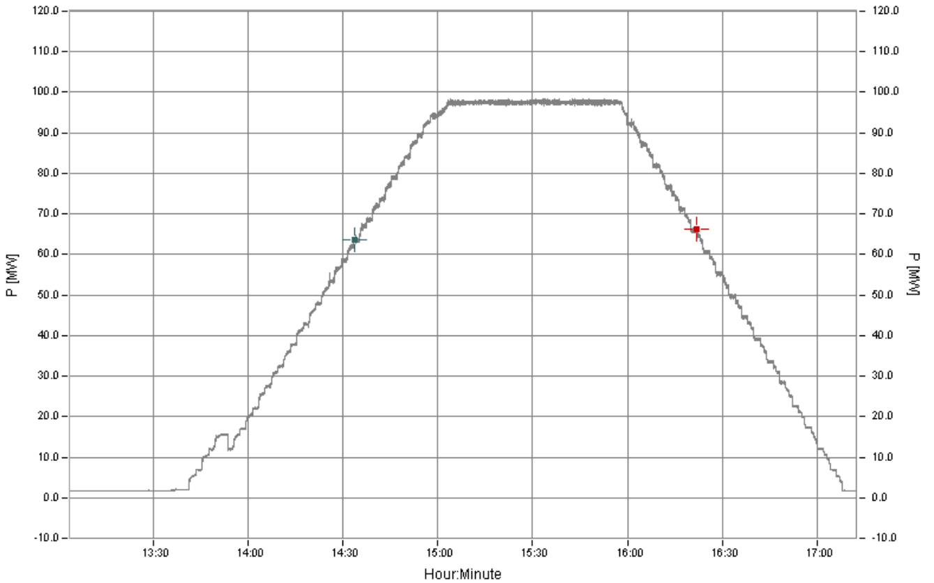
a. Total power at load 100MW
