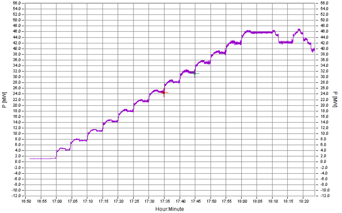
b. Power consumption at speed 200 rpm
