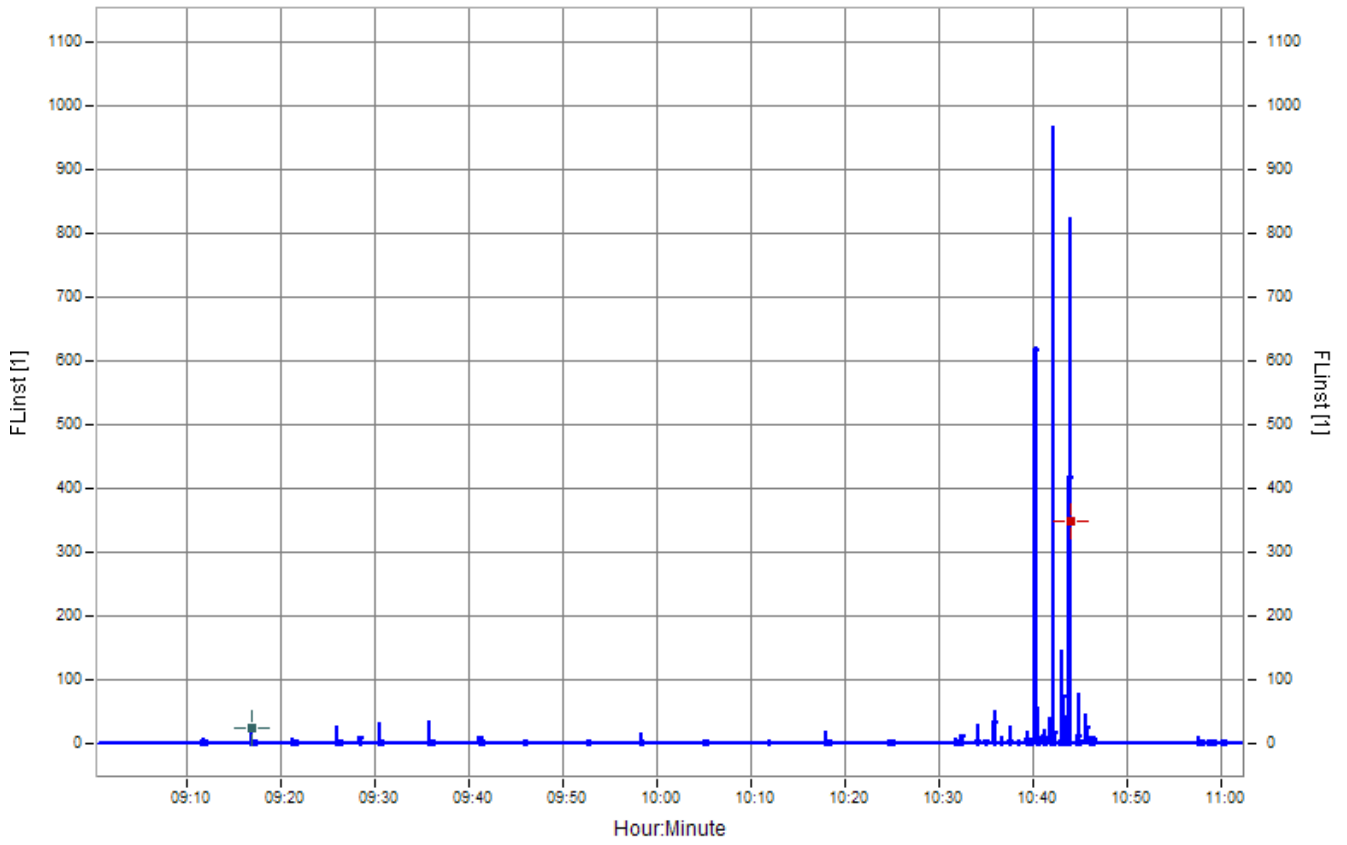
b. Instantaneous Flicker
